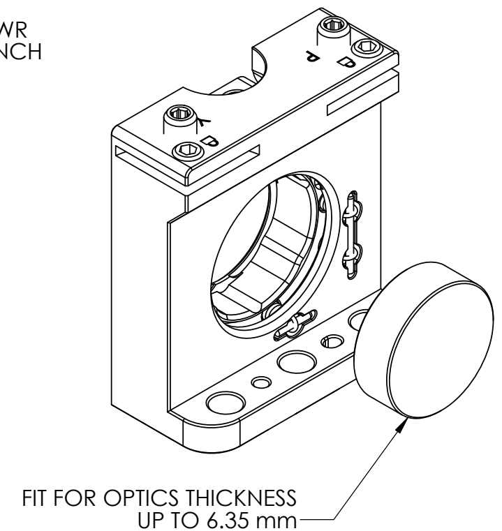
MODEL: HVM-075r REAR LOAD
