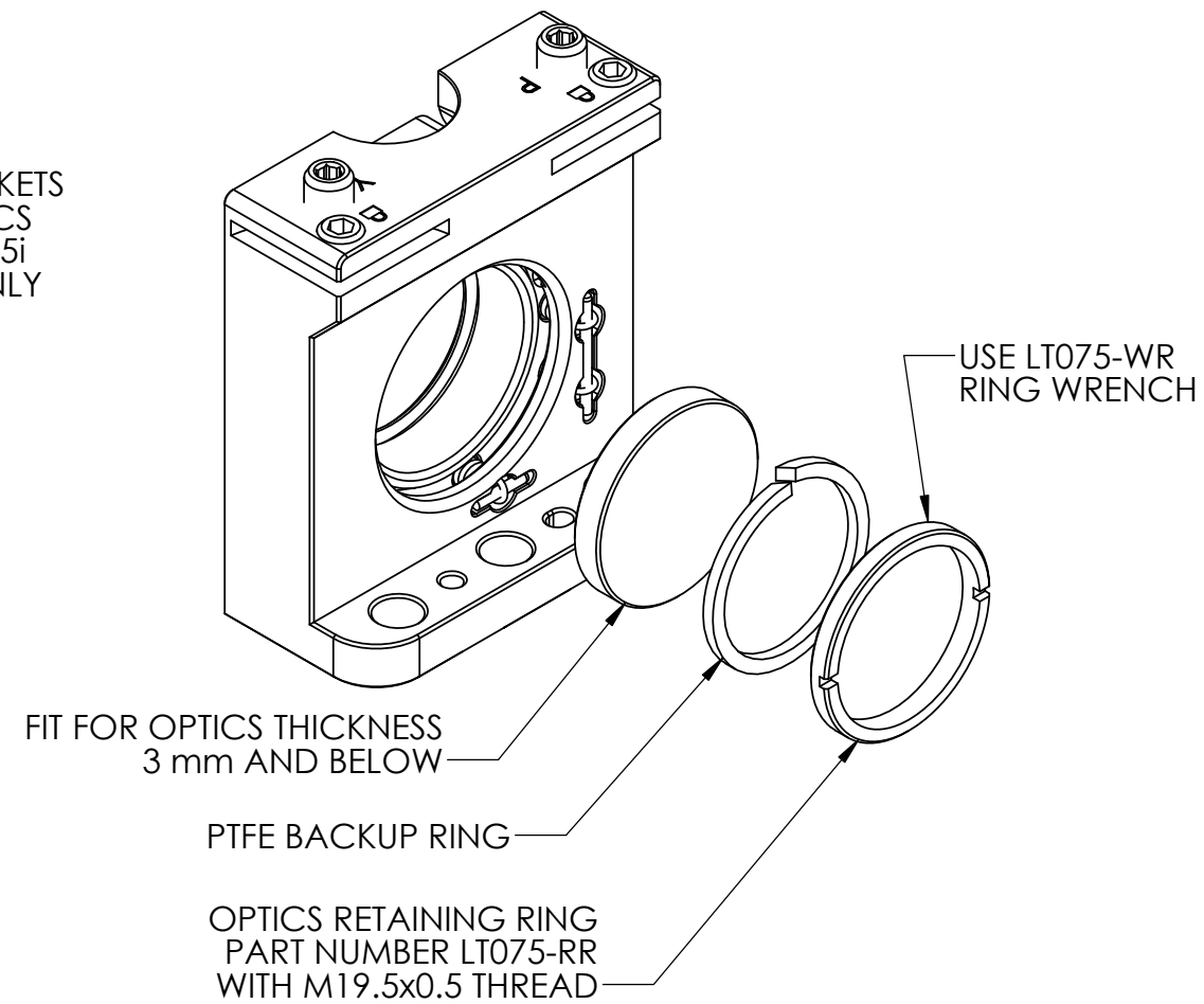
MODEL: HVM-075i REAR LOAD THREADED BORE
